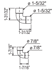
<Elbow pipe (Accessory)>
