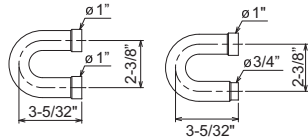
<Low-pressure pipe twining kit (Accessory)>
