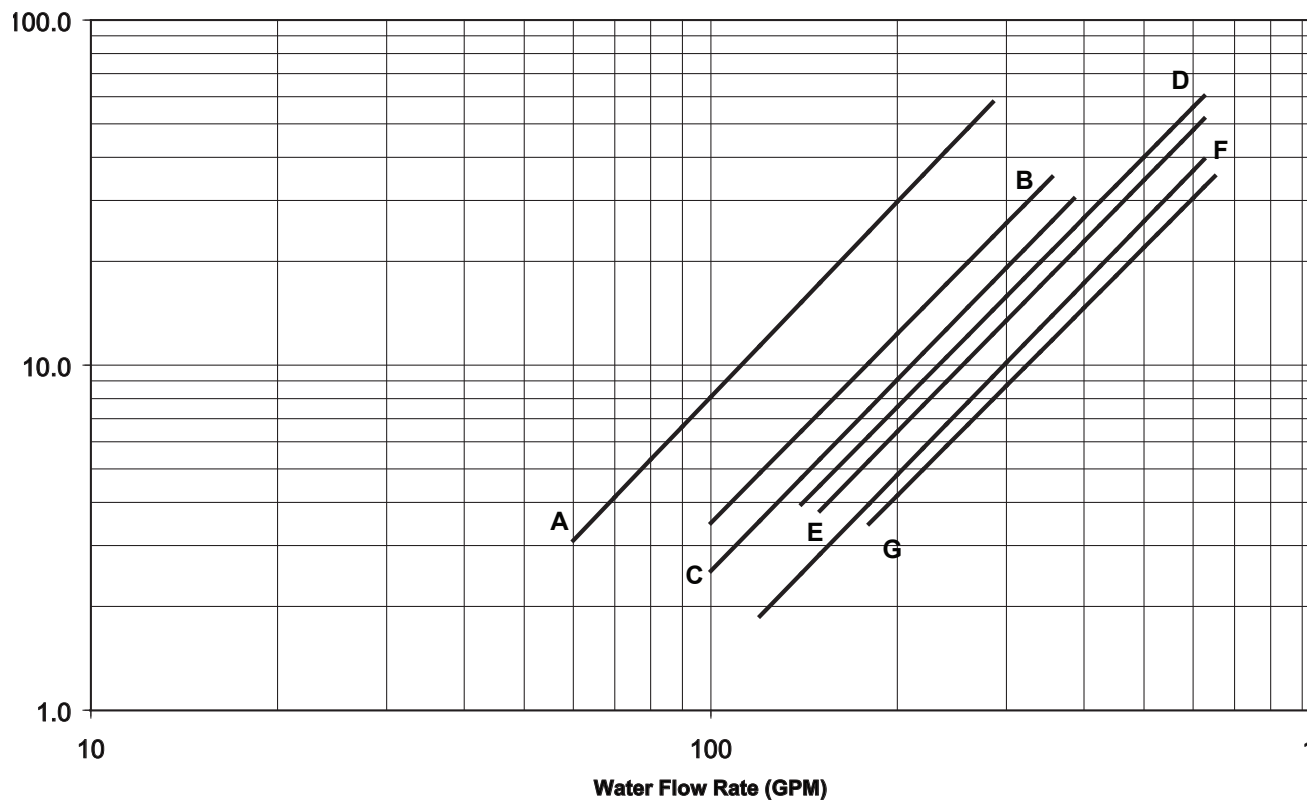
YLAA Evaporator Pressure Drop (IP Units)
